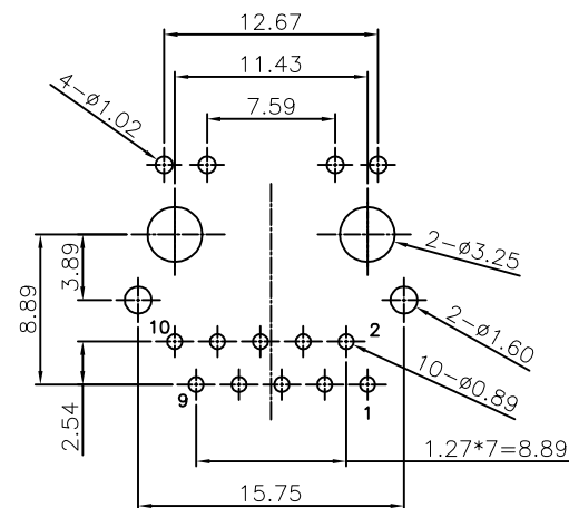
RECOMMENED PCB LAYOUT COMPONENT SIDE TOLERANCE ±0.05
